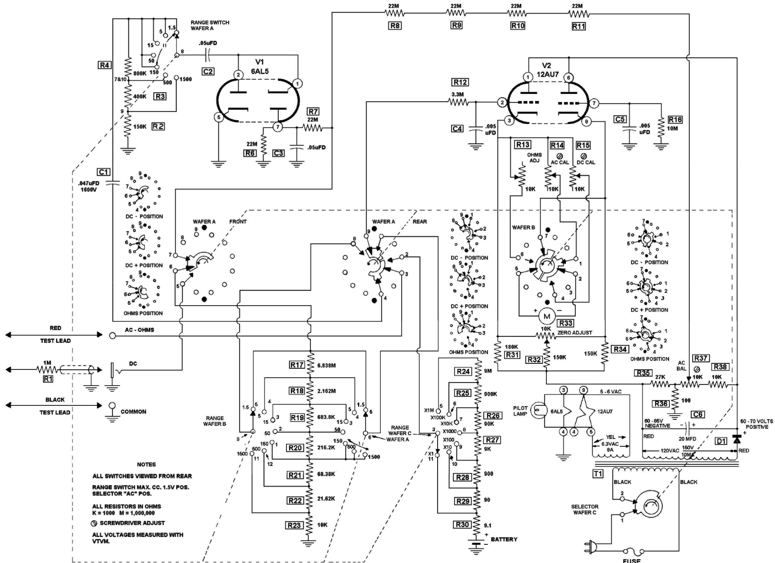
SCHEMATIC OF THE HEATHKIT SERVICE BENCH VTVM MODEL IM-10
